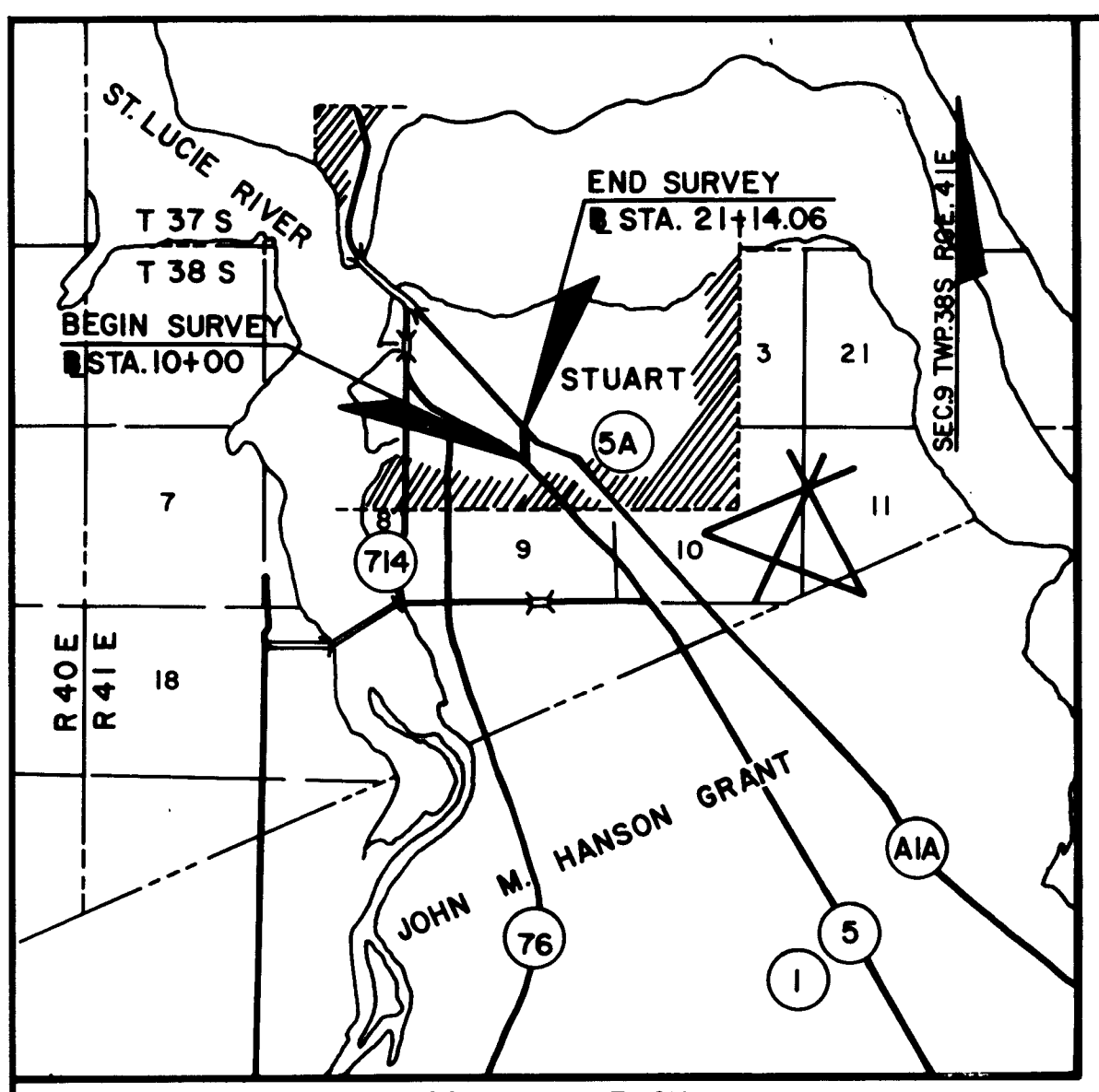
LOCATION SKETCH SCALE 1" = 1 MILE
